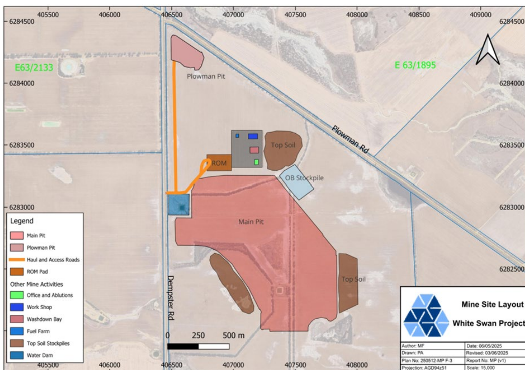
Figure 2: White Swan Kaolin Project Mining Development and Closure Proposal Site Layout as approved
